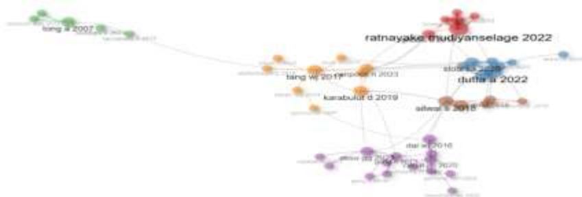
Figure 15. Co-citation network
